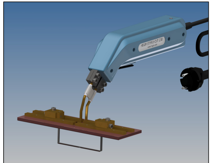
Profile cut adapter with HSGM-Styro-Cut-230 (HSGM-Styro-Cut 230 and cutting band not included in scope of delivery!)
